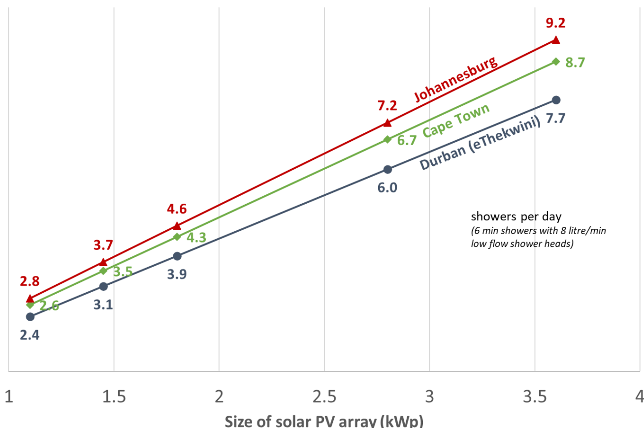
Average no. of showers per day for different solar PV array sizes
