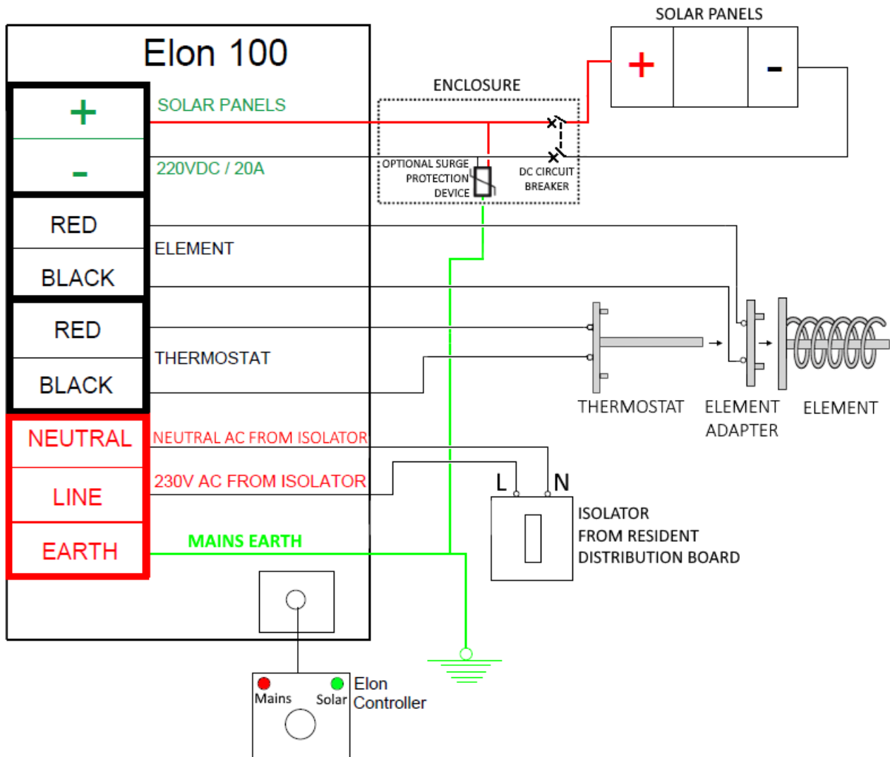
Wiring diagram: Elon 100 with element adapter:
